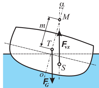
Obr. 47 Stabilita
